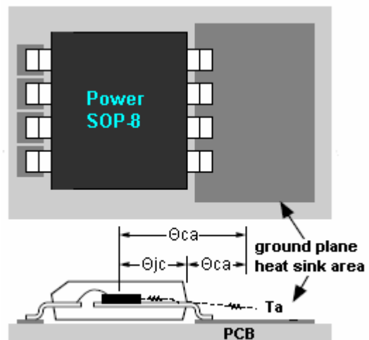
Thermal Resistance
