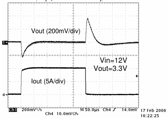
Figure 4. Load Step Response: 0->10A
