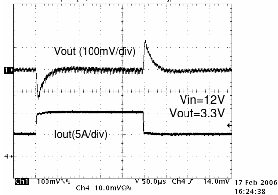
Figure 3. Load Step Response: 5->10A
