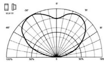
Directive Characteristics
