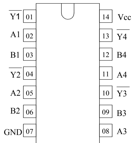
Figure 1 – Pinout
