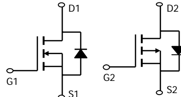
n-channel
