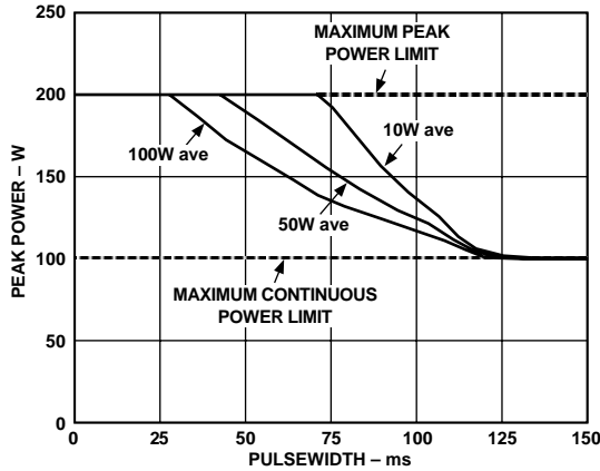
Figure 17. Largest On-State Power vs. Pulswidth that Maintains T_{JMAX} \leq 110^{\circ}C at 90^{\circ}C Baseplate
