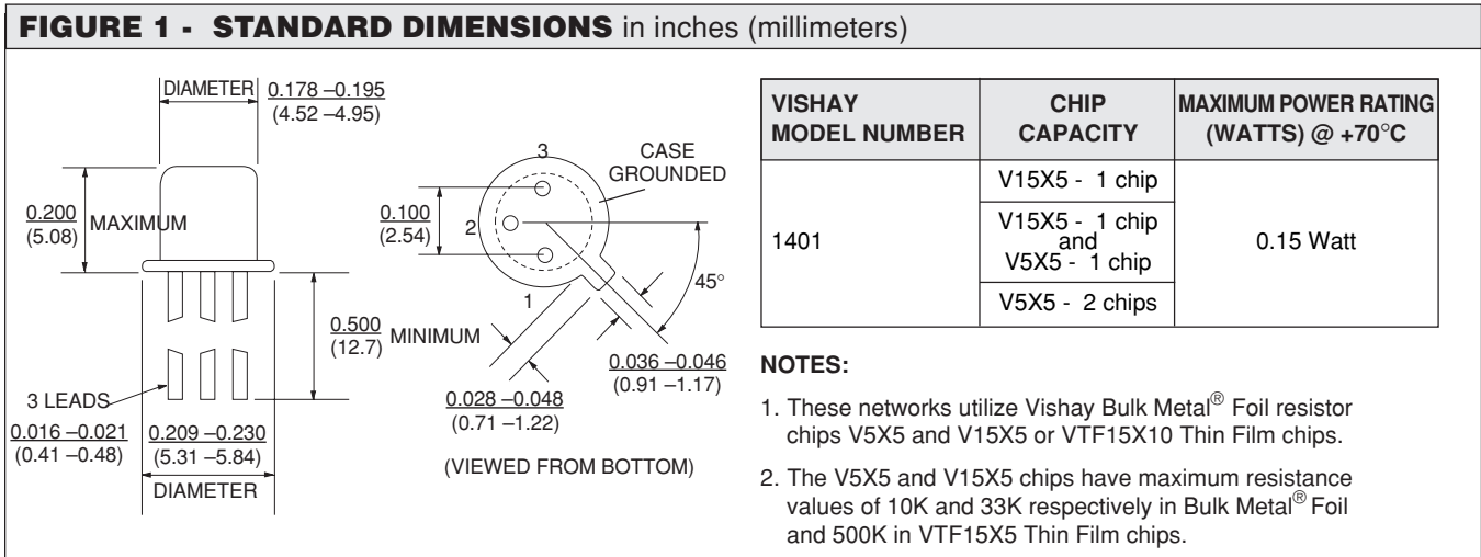
3 pins on a 0.100" pin circle— pin 3 case grounded .
