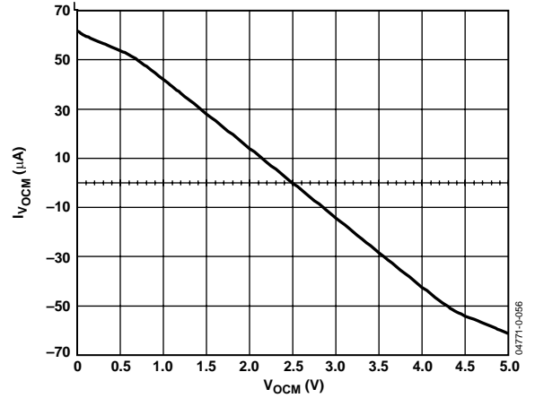
Figure 53. V OCM Bias Current vs. V OCM Input Voltage
