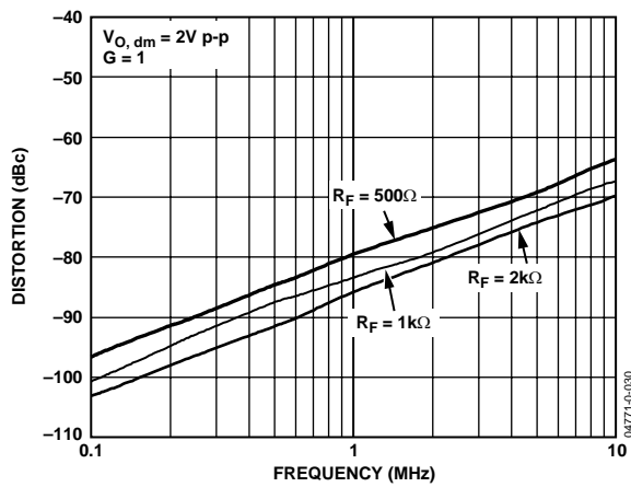
Figure 27. Second Harmonic Distortion at Various R_F
