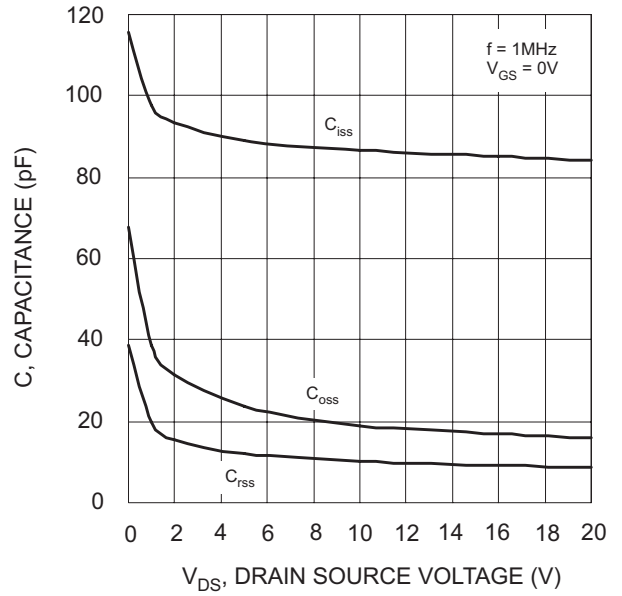
Fig. 12 Capacitance Variation
