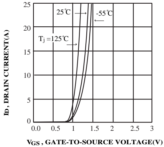
FIG.2 Transfer Characteristics
