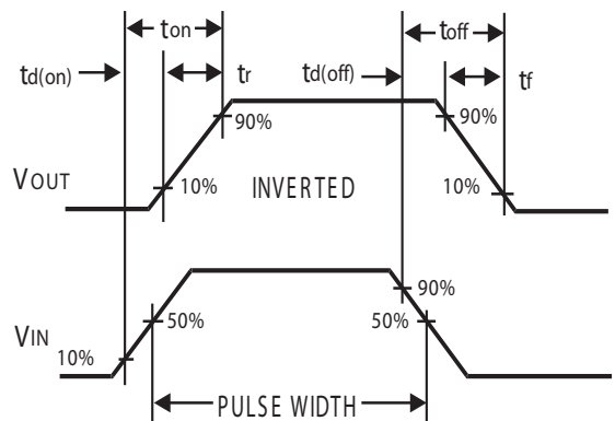
FIG.12 Switching Waveforms
