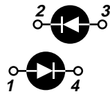
Anti-Parallel APT2X30D60J
