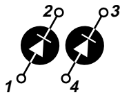
Parallel APT2X31D60J
