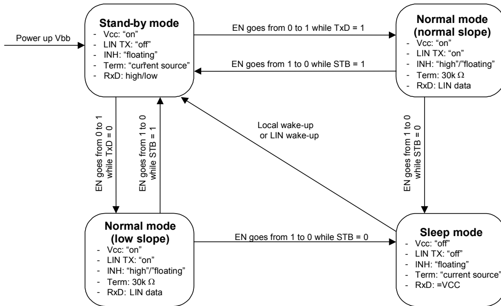
Figure 4: State Diagram
