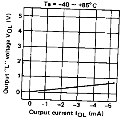
Output "L" voltage ( V_{OL} ) vs. output current ( I_{OL} )
