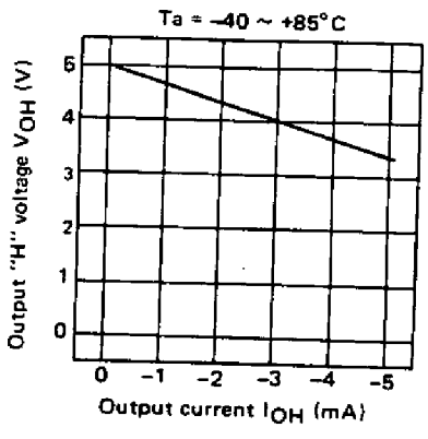
Output "H" voltage ( V_{OH} ) vs. output current ( I_{OH} )
