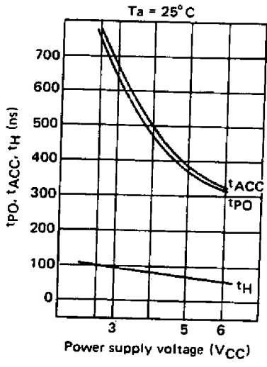
t_{PO} , t_H , and t_{ACC} vs. power supply voltage ( V_{CC} )
