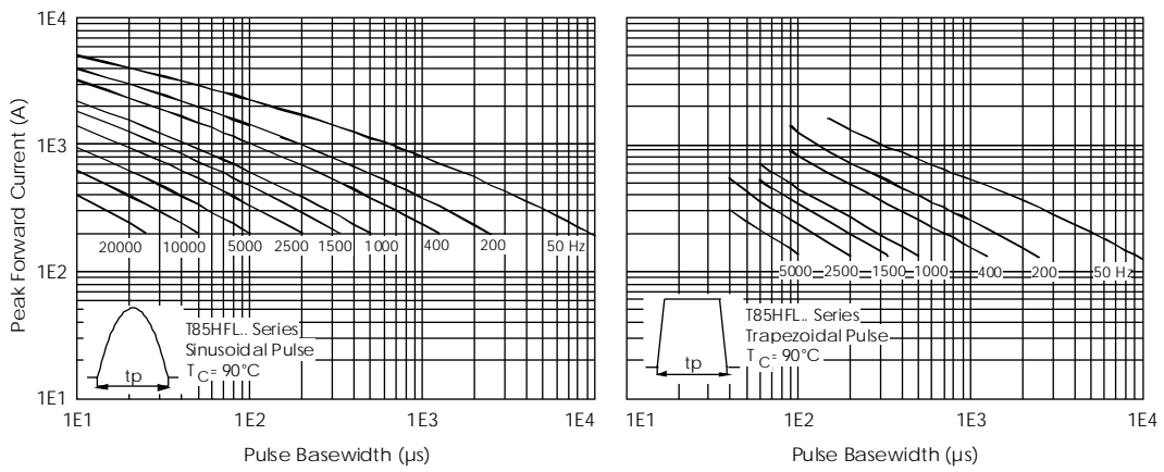
Fig. 44 - Frequency Characteristics
