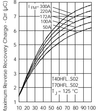
Fig. 20 - Recovery Charge Characteristics
