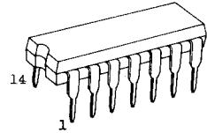
DIP14 (3D14A-P)
