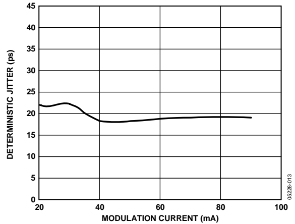
Figure 15. Deterministic Jitter at 2.488 Gbps vs. Modulation Current, I_{BIAS} = 20 mA
