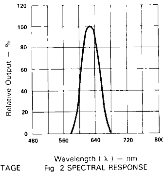
Fig 2 SPECTRAL RESPONSE
