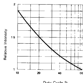
Fig 6 LUMINOUS INTENSITY Vs DUTY CYCLE % (AVERAGE I_F = 10 \text{ mA} PER SFG)
