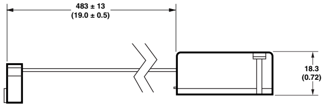
HEDL-550X/554X/560X/564X HEDL-556X/557X
