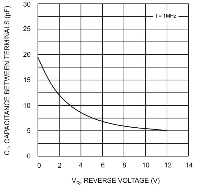
Fig. 4 Typical Capacitance Between Terminals Characteristics
