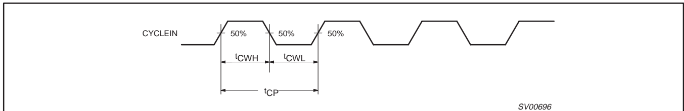
Figure 41. CYCLEIN Waveform
