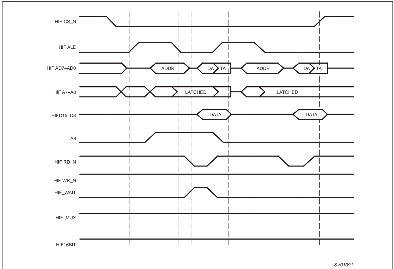
Figure 9. 16 Bit Read Cycle Multiplexed
