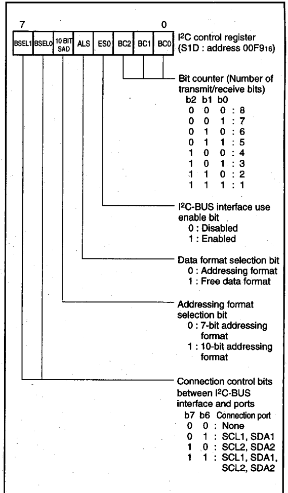
Fig. 38. Structure of I 2 C control register
