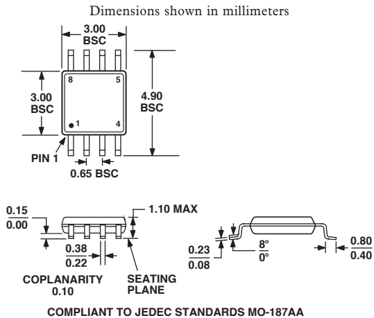
8-Lead MSOP Package [MSOP] (RM-8)
