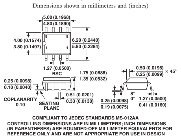
8-Lead Standard Small Outline Package [SOIC] Narrow Body (RN-8)
