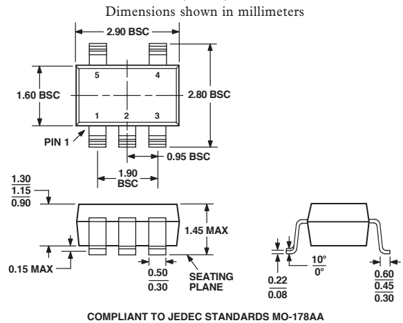
5-Lead Plastic Surface-Mount Package [SOT-23] (RT-5)
