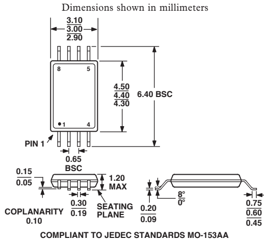
8-Lead Thin Shrink Small Outline Package [TSSOP] (RU-8)
