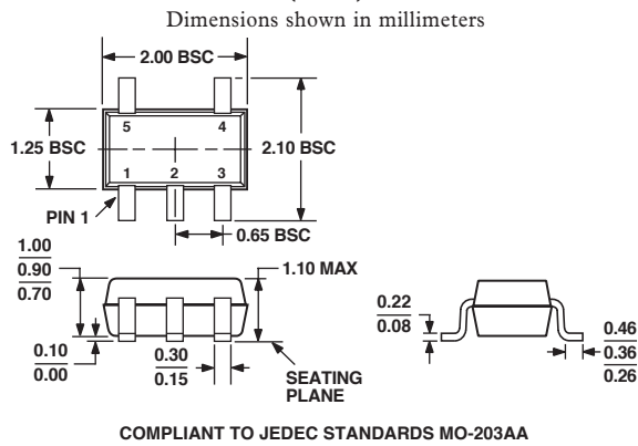
5-Lead Plastic Surface Mount Package [SC70] (KS-5)
