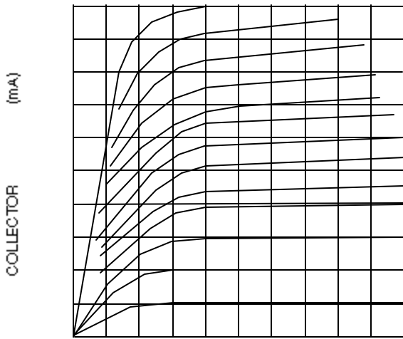
COLLECTOR CURRENT Collector Current vs. Collector Voltage
