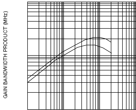
COLLECTOR CURRENT Gain-Bandwidth Product vs. Collector Current
