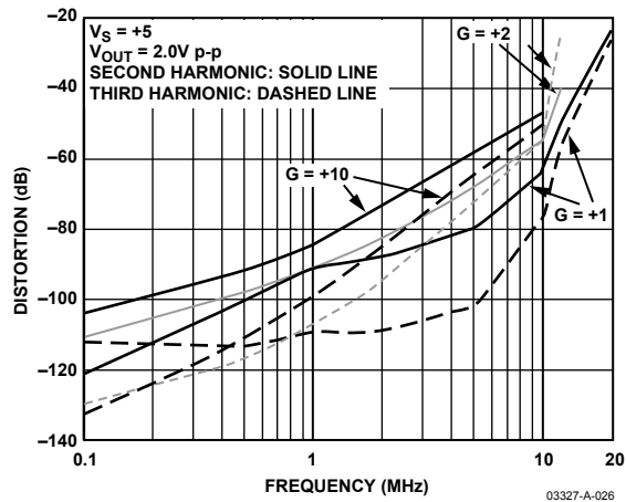
Figure 27. Harmonic Distortion vs. Frequency and Gain
