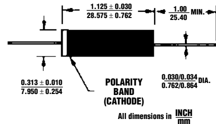
FIGURE 1 DESIGN DATA
