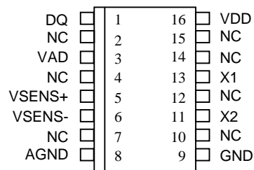
16-PIN SSOP
