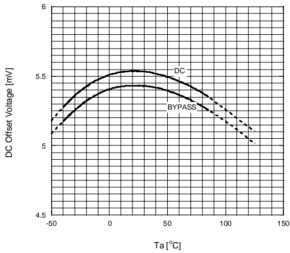
DC Offset Voltage vs. Temperature V_{+}=12V, V_{out}=Rch
