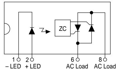
CPC1965Y Pinout
