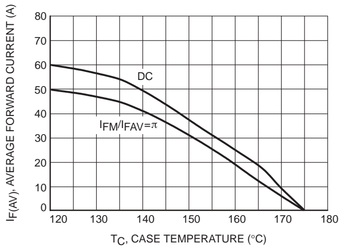
Figure 4. Current Derating
