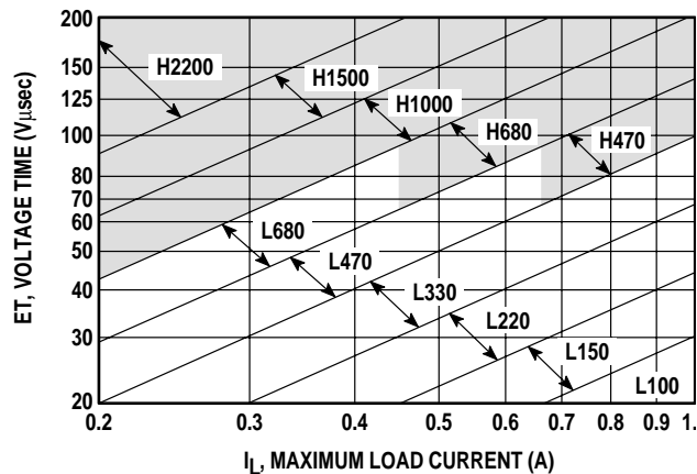
Figure 35. TC2575-Adj
