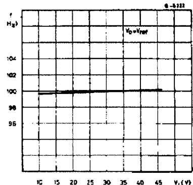
Figure 11. Switching frequency vs. input voltage
