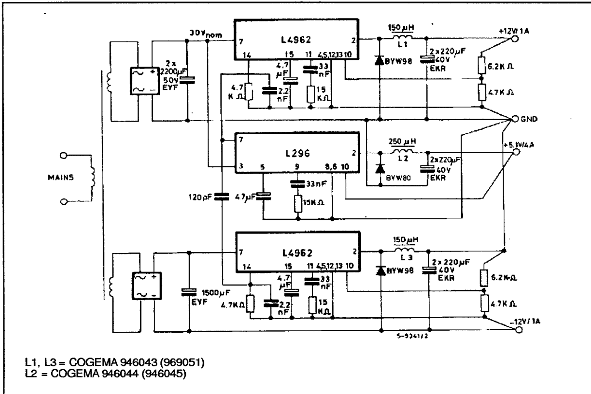
Figure 29. DC-DC converter 5.1V/4A, ±12V/1A. A suggestion how to synchronize a negative output
