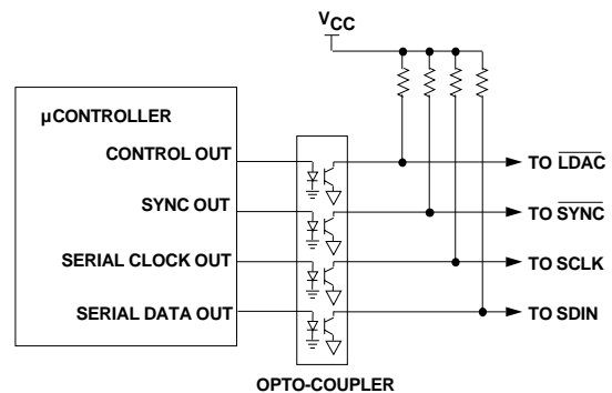
Figure 19. Opto-Isolated Interface.
