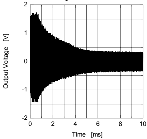
AGC Attack Time (C:9pin=0.47 μF)
