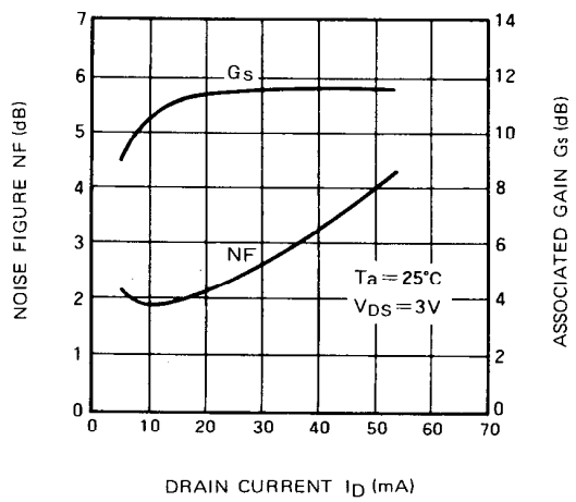
NF & G_s vs. I_D ( f = 12\text{ GHz} )
