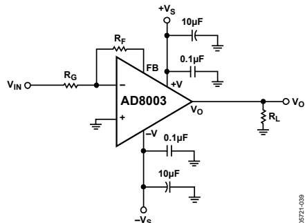
Figure 39. Inverting Gain
