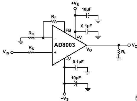
Figure 38. Noninverting Gain
