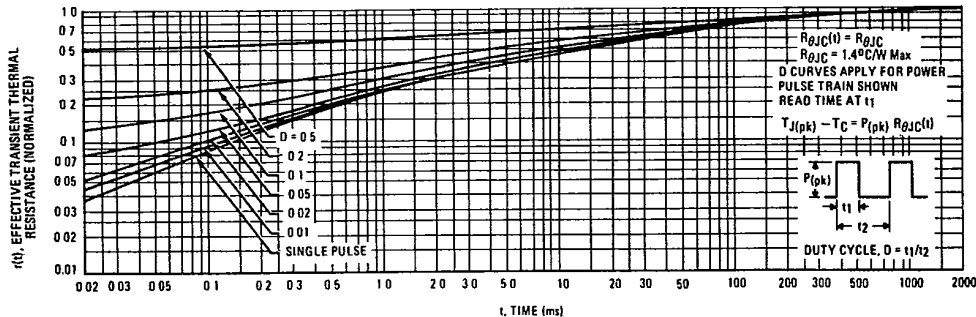
FIGURE 11 — THERMAL RESPONSE
