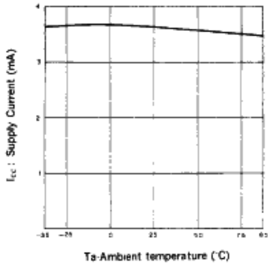
Supply current vs. temperature ( V_{CC}=5V, SW, MOD supply current included)
