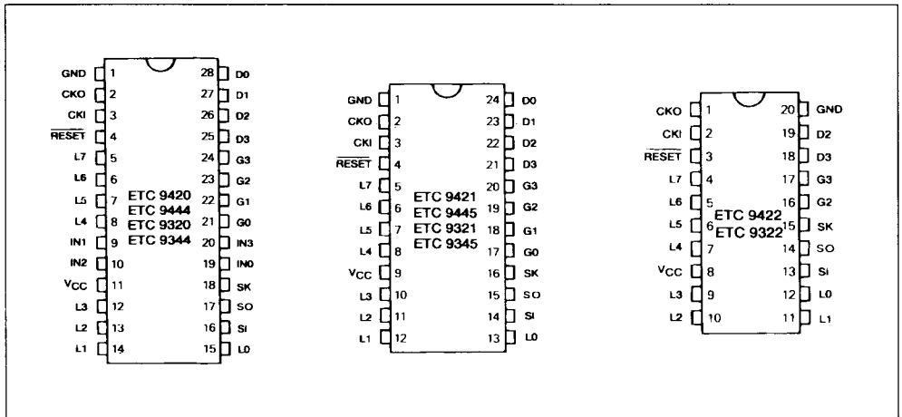
Figure 2 : Pins Connections.
