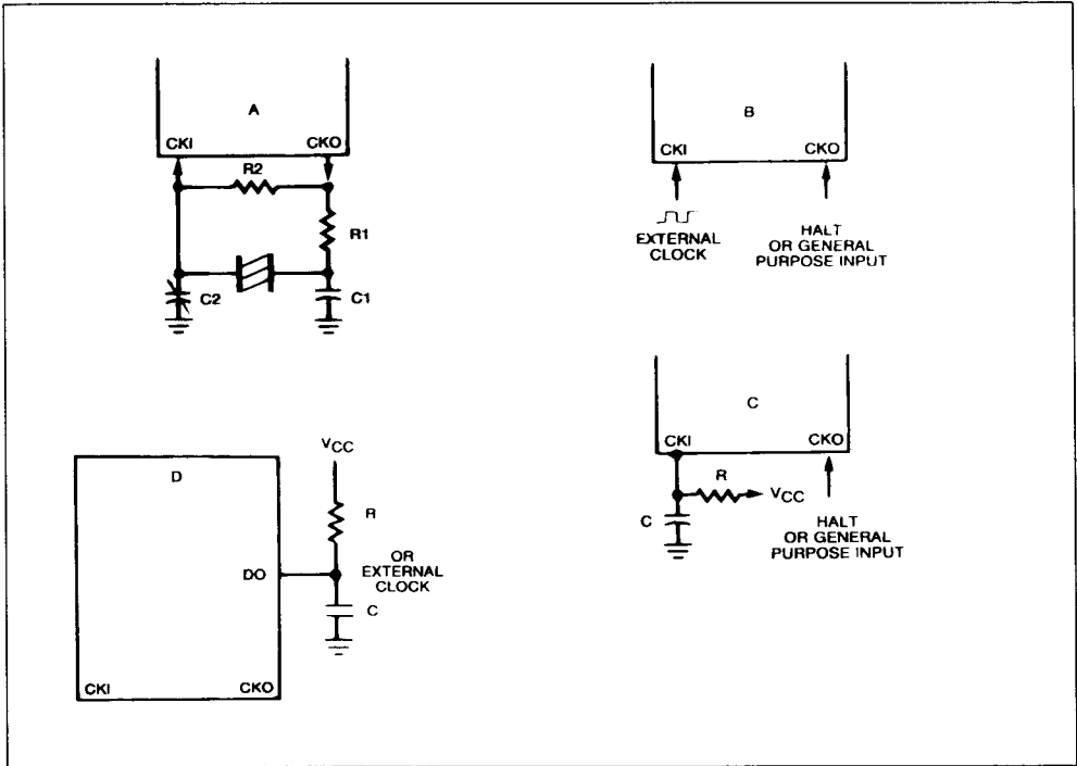
Figure 8 : Oscillator Components Values.
