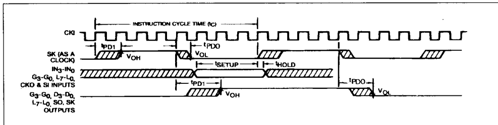
Figure 4 : Microbus Read Operation Timing.
