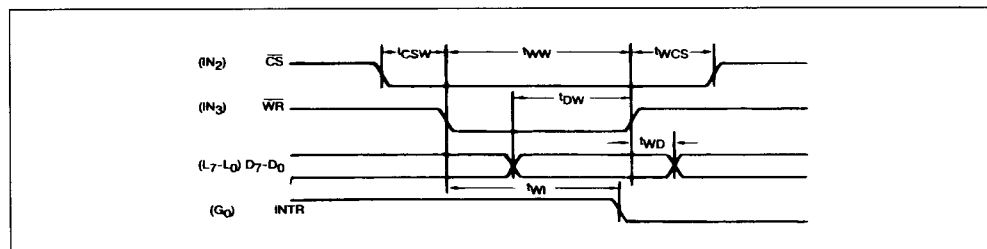
Figure 5 : Microbus Write Operation Timing.
