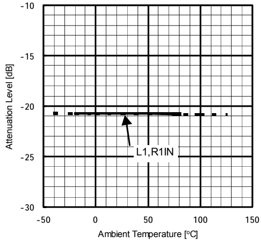
Attenuation Level vs. Ambient Temperature V^+=12V, V_{in}=1V, f=1kHz, Vol=-20dB
