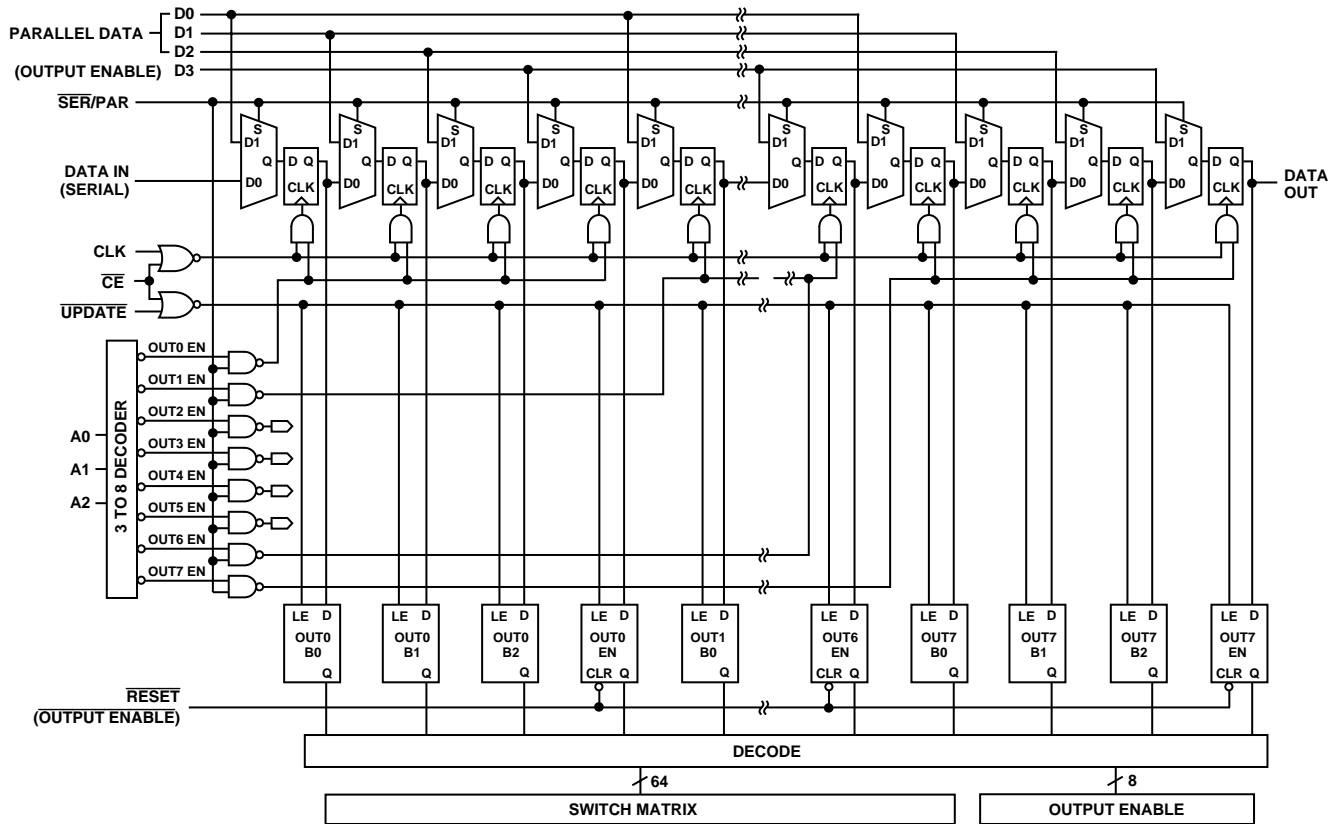
Figure 4. Logic Diagram
