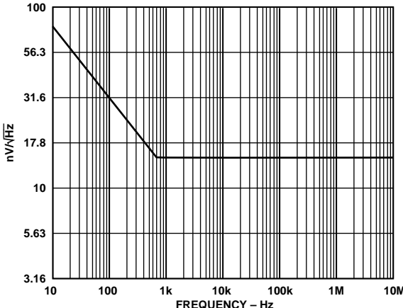
Figure 19. AD8108 Voltage Noise vs. Frequency
