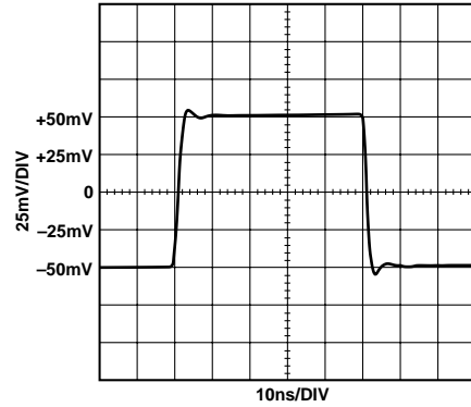
Figure 15. AD8109 Step Response, 100 mV Step
