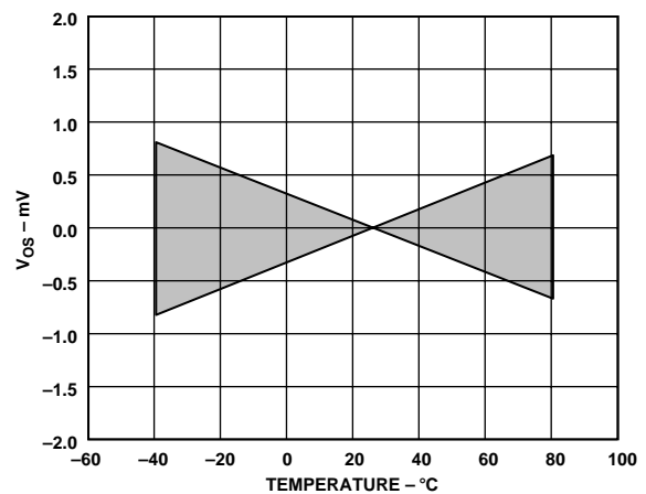
Figure 41. AD8109 Offset Voltage Drift vs. Temperature (Normalized at +25°C)
