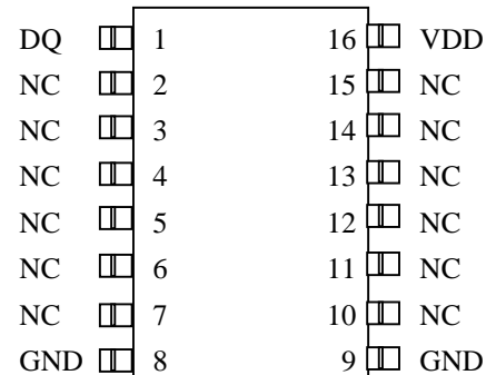
DS2434 16-Pin SSOP See Mech. Drawings Section
