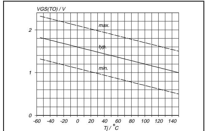
Fig. 10. Gate threshold voltage. V_{GS(TO)} = f(T_j) ; conditions: I_D = 1 mA; V_{DS} = V_{GS}
