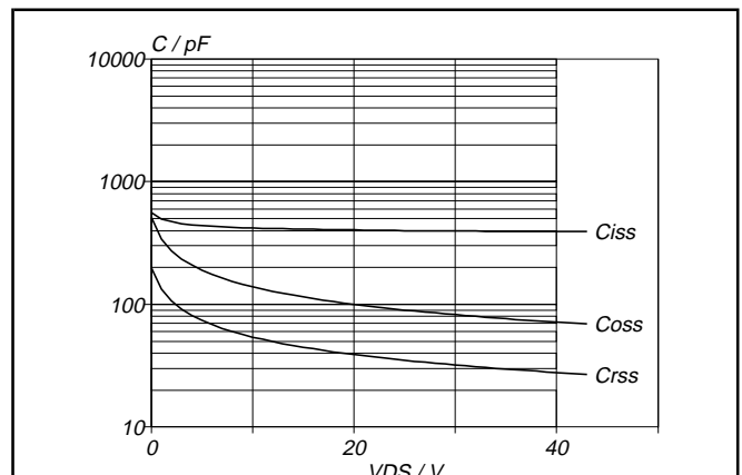
Fig. 12. Typical capacitances, C_{iss} , C_{oss} , C_{rss} . C = f(V_{DS}) ; conditions: V_{GS} = 0 V; f = 1 MHz
