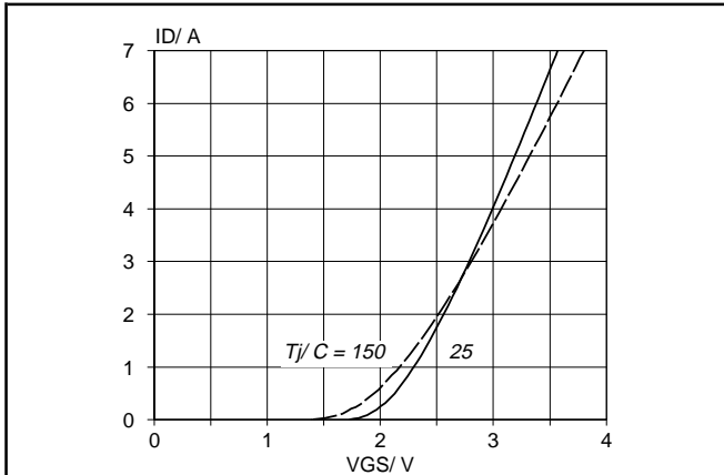
Fig. 7. Typical transfer characteristics. I_D = f(V_{GS}) ; conditions: V_{DS} = 25 V; parameter T_j
