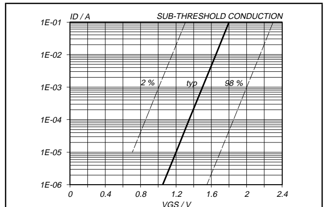
Fig. 11. Sub-threshold drain current. I_D = f(V_{GS}) ; conditions: T_j = 25 ^{\circ}C ; V_{DS} = V_{GS}
