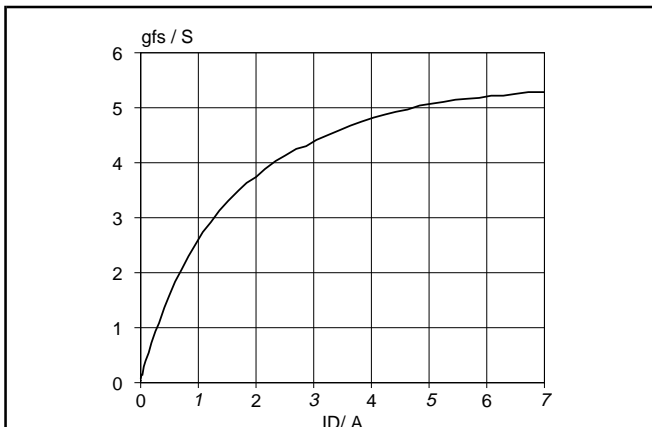
Fig. 8. Typical transconductance, T_j = 25 ^{\circ}C . g_{fs} = f(I_D) ; conditions: V_{DS} = 25 V
