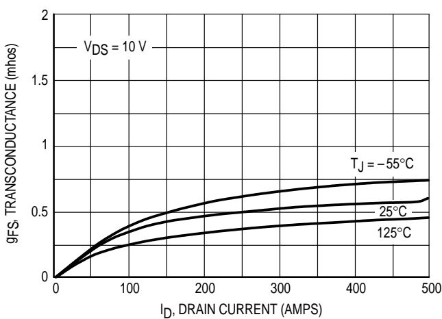
Figure 8. Transconductance
