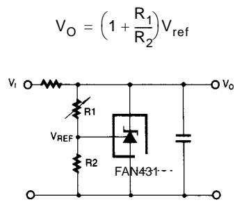
Figure 13. Shunt Regulator
