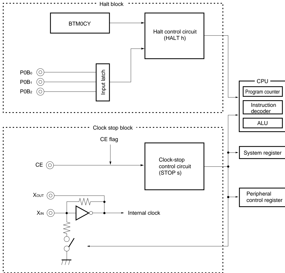
Fig. 14-1 Standby Block
