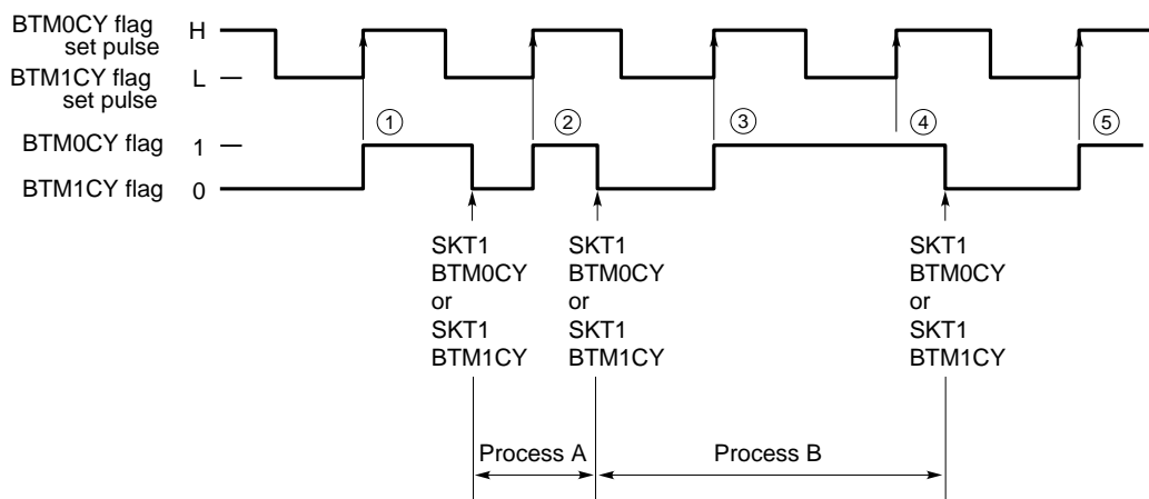
Fig. 10-5 Detection of the BTM0CY and BTM1CY Flags
