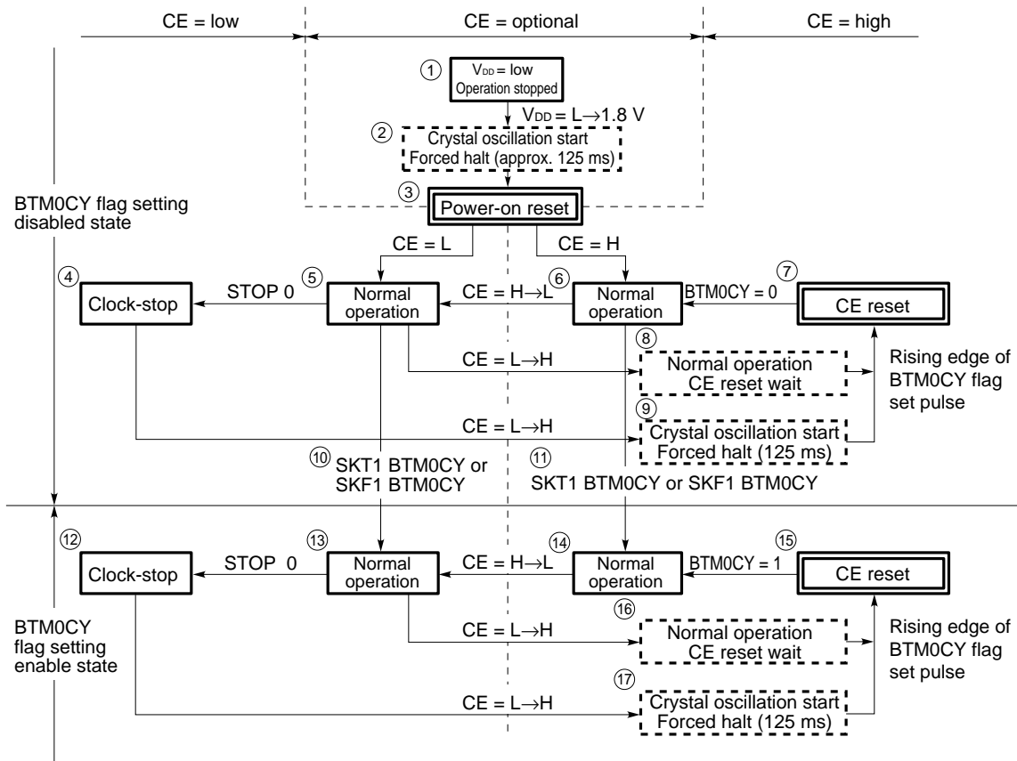
Fig. 15-8 BTM0CY Flag State Transition
