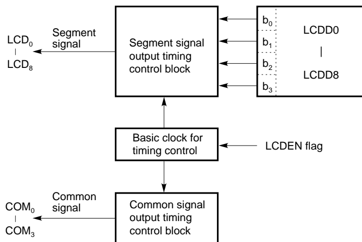
Fig. 13-6 Configuration and Functions of LCD Enable Register
