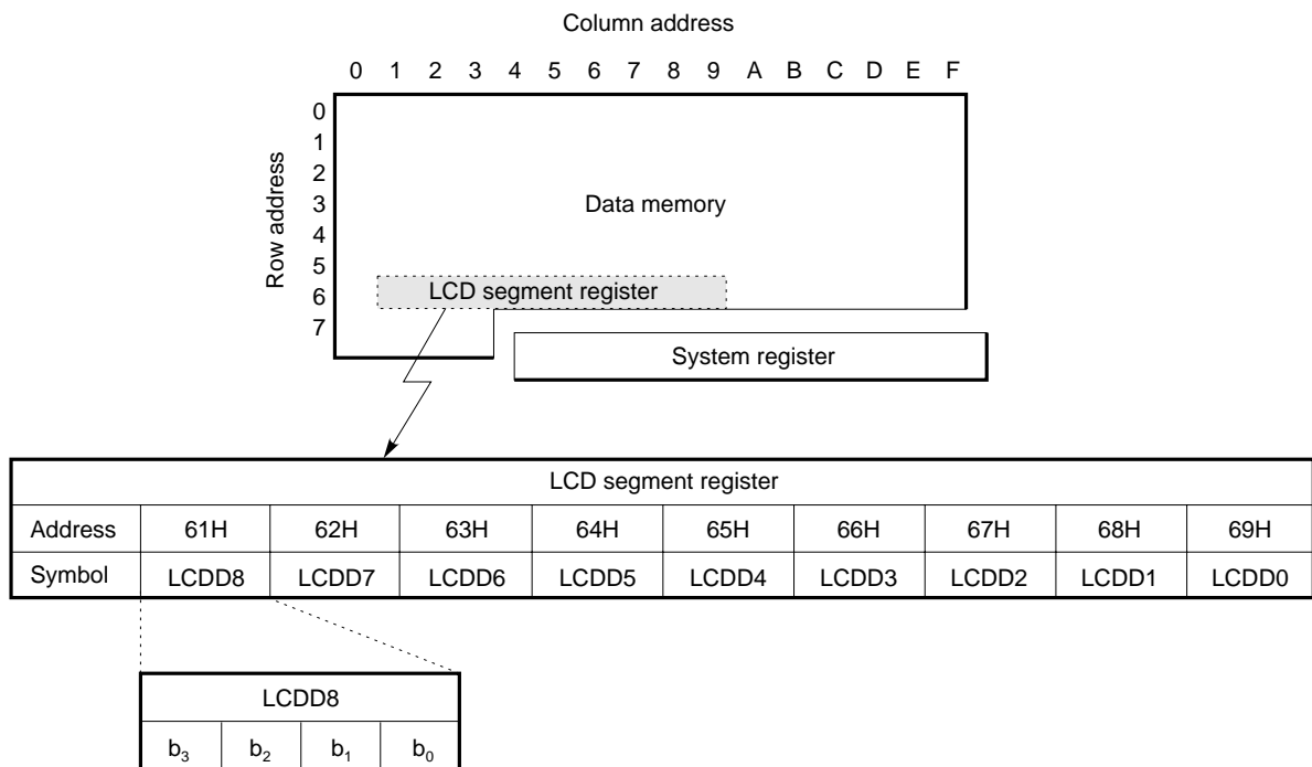
Fig. 13-3 Configuration of LCD Segment Register in Data Memory
