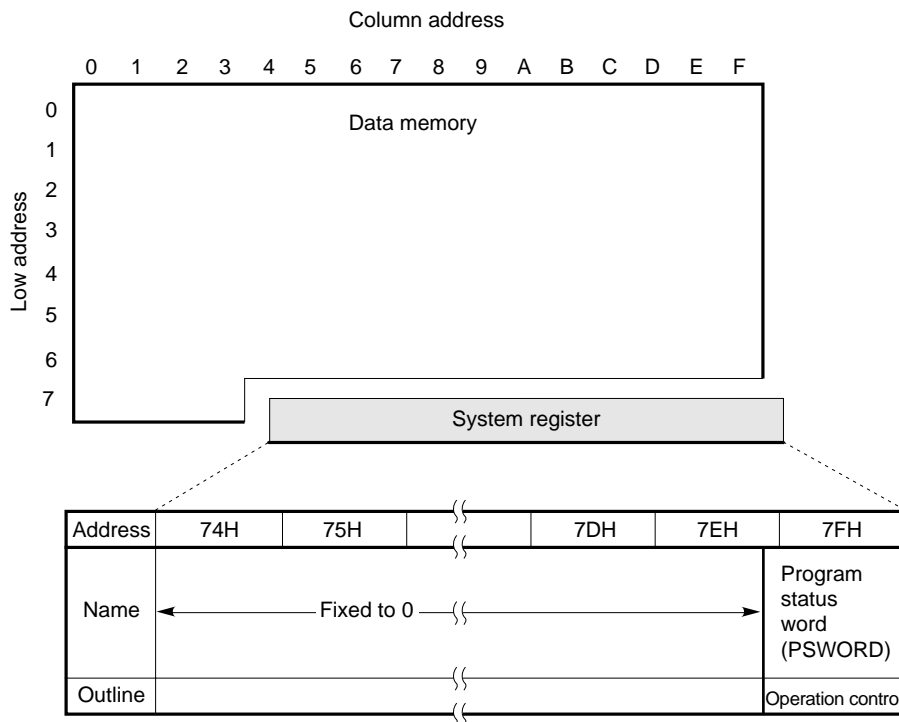
Fig. 5-1 Location on Data Memory and Outline of System Registers
