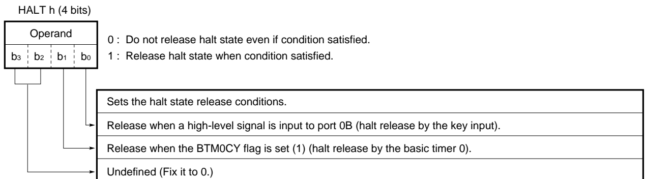
Fig. 14-2 Halt Release Conditions
