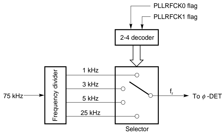
Fig. 11-5 Reference Frequency Generator
