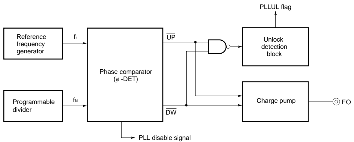
Fig. 11-6 Phase Comparator, Charge Pump and Unlock Detection Block
