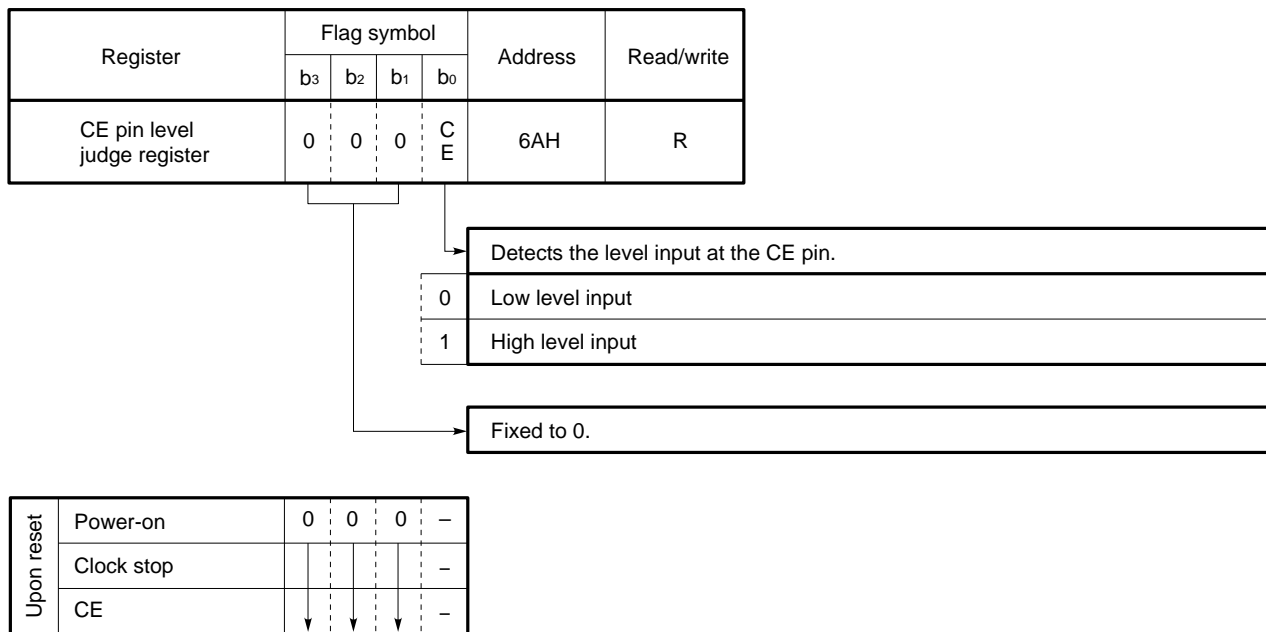
Fig. 14-6 Configuration of CE Pin Level Judge Register
