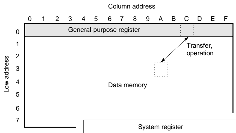
Fig. 6-1 Outline of General-Purpose Register
