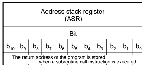
Fig. 3-1 Configuration of Address Stack Registers
