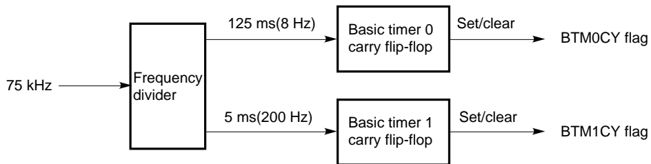
Fig. 10-1 Overview of Timers
