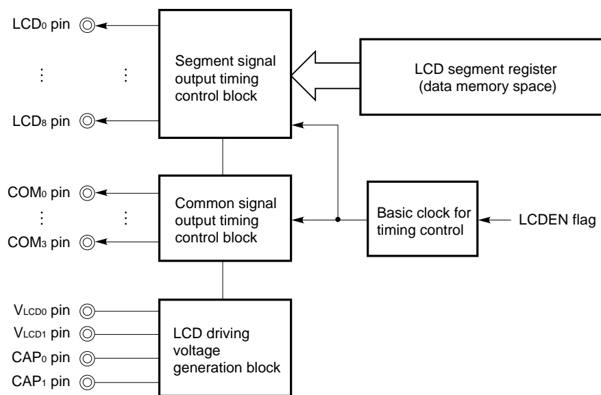
Fig. 13-1 Overview of LCD Controller/Driver
