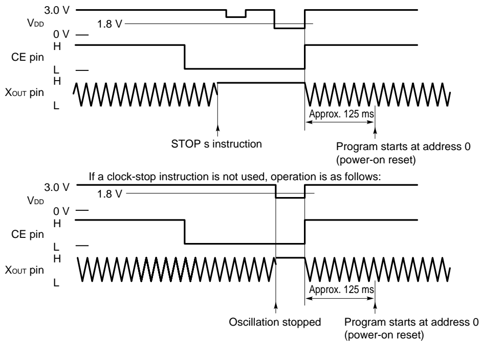
Fig. 14-4 Clock-Stop Release by Power-On Reset (T A = -10 to +50 °C)
