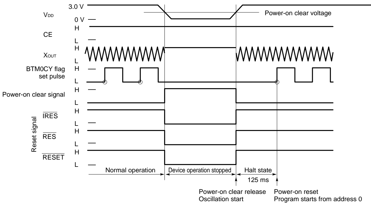
Fig. 15-2 Power-On Reset Operation
