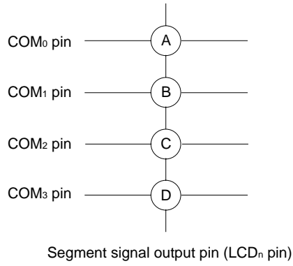
Fig. 13-7 Common Signal and Segment Signal Output Waveforms
