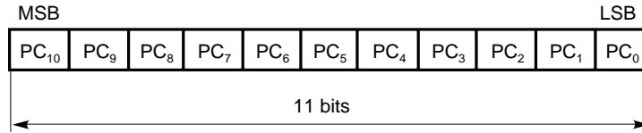
Fig. 2-3 Program Counter Configuration
