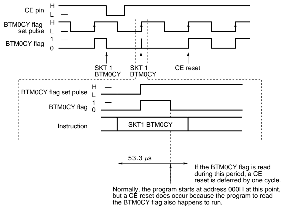
Fig. 10-7 Operation That Occurs If a CE Reset Occurs Simultaneously with a BTM0CY Flag Read Instruction
