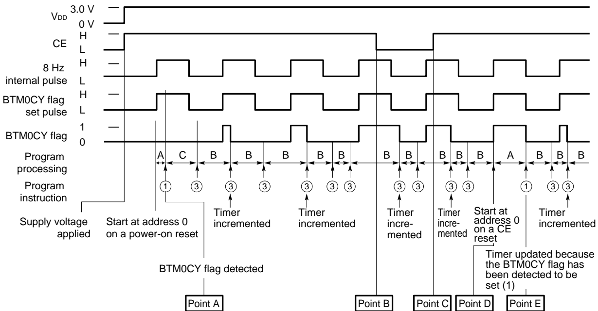
Fig. 10-6 Timing Chart
