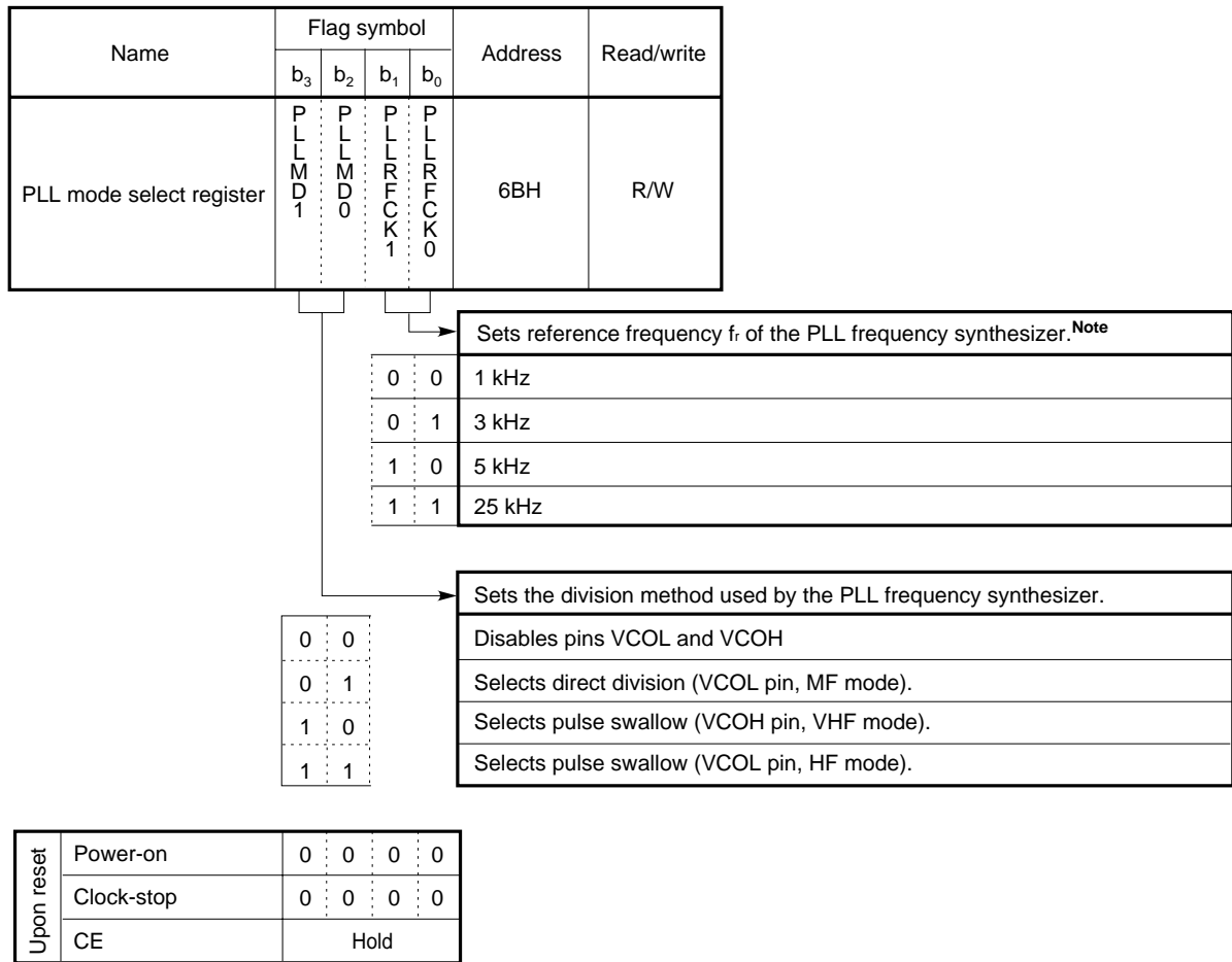
Fig. 11-3 Configuration and Functions of the PLL Mode Select Register
