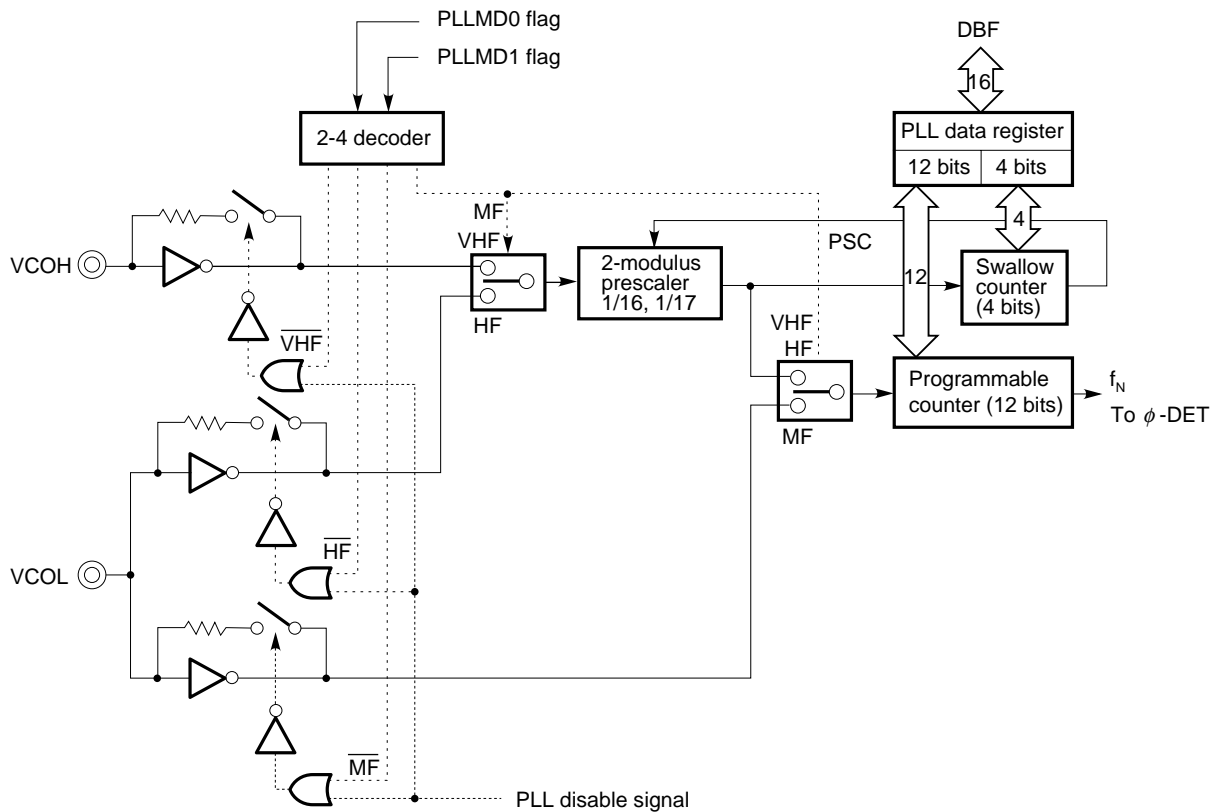
Fig. 11-2 Input Switching Block and Programmable Divider
