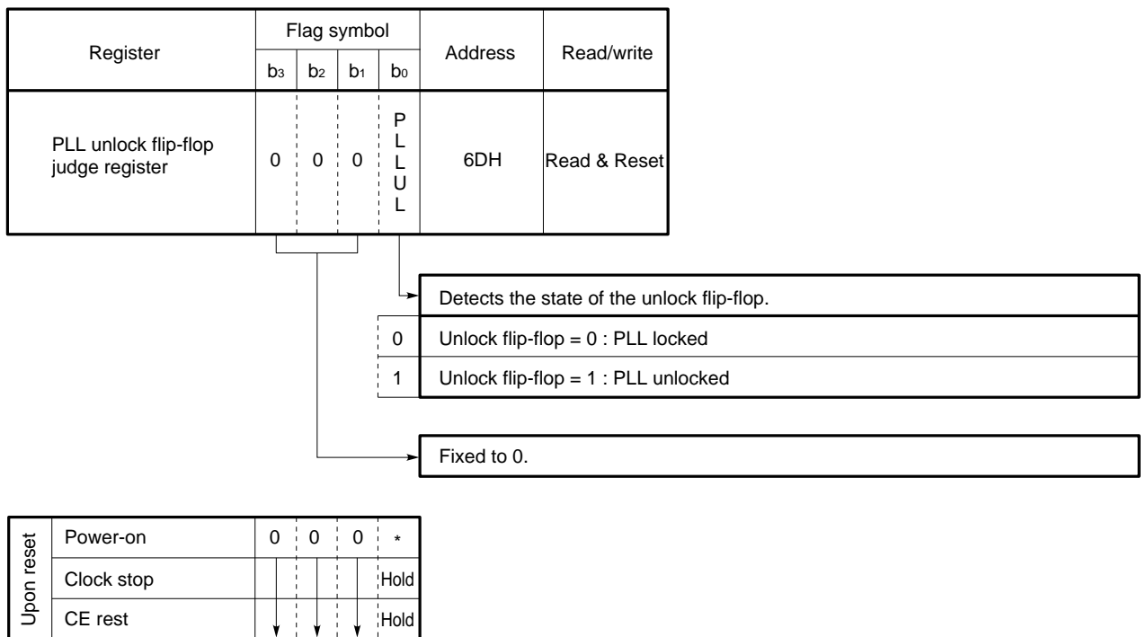
Fig. 11-8 Configuration and Functions of PLL Unlock Flip-Flop Judge Register
