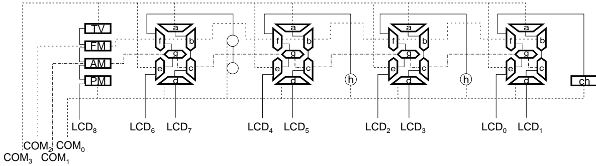
Fig. 13-8 Example of LCD Panel Connection
