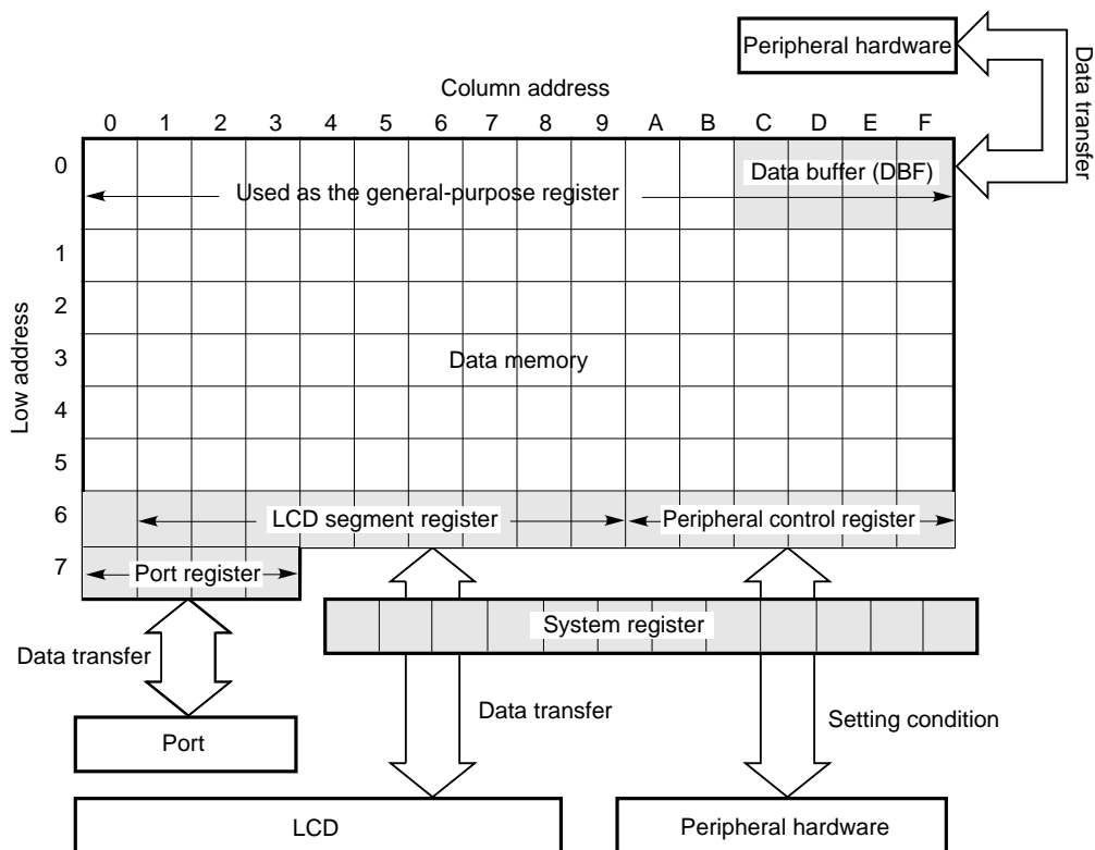
Fig. 4-1 Outline of Data Memory
