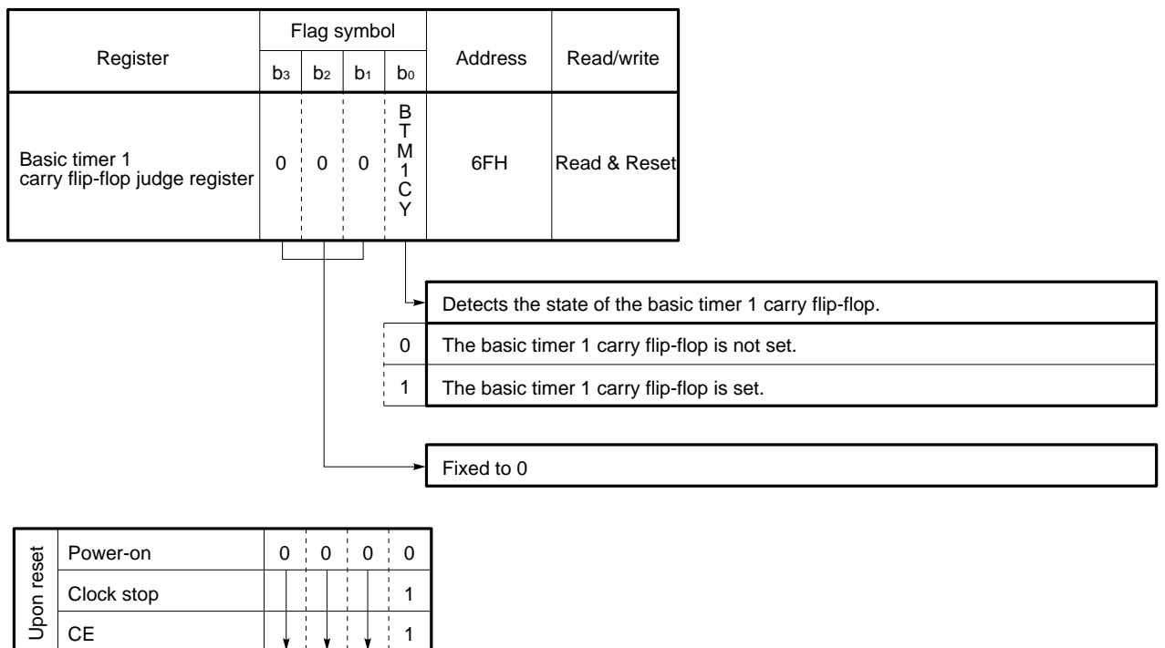
Fig. 10-3 Configuration of the Basic Timer 1 Carry Flip-Flop Judge Register
