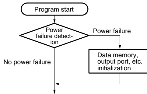
Fig. 15-7 Power Failure Detection Flowchart
