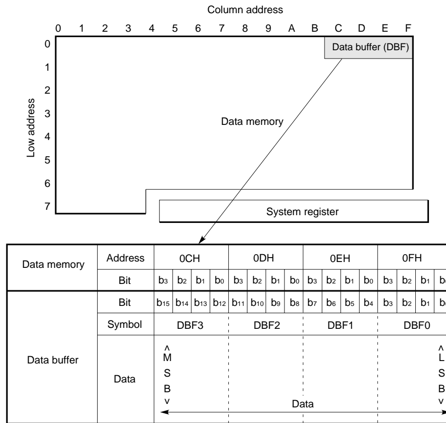
Fig. 8-2 Configuration of the Data Buffer
