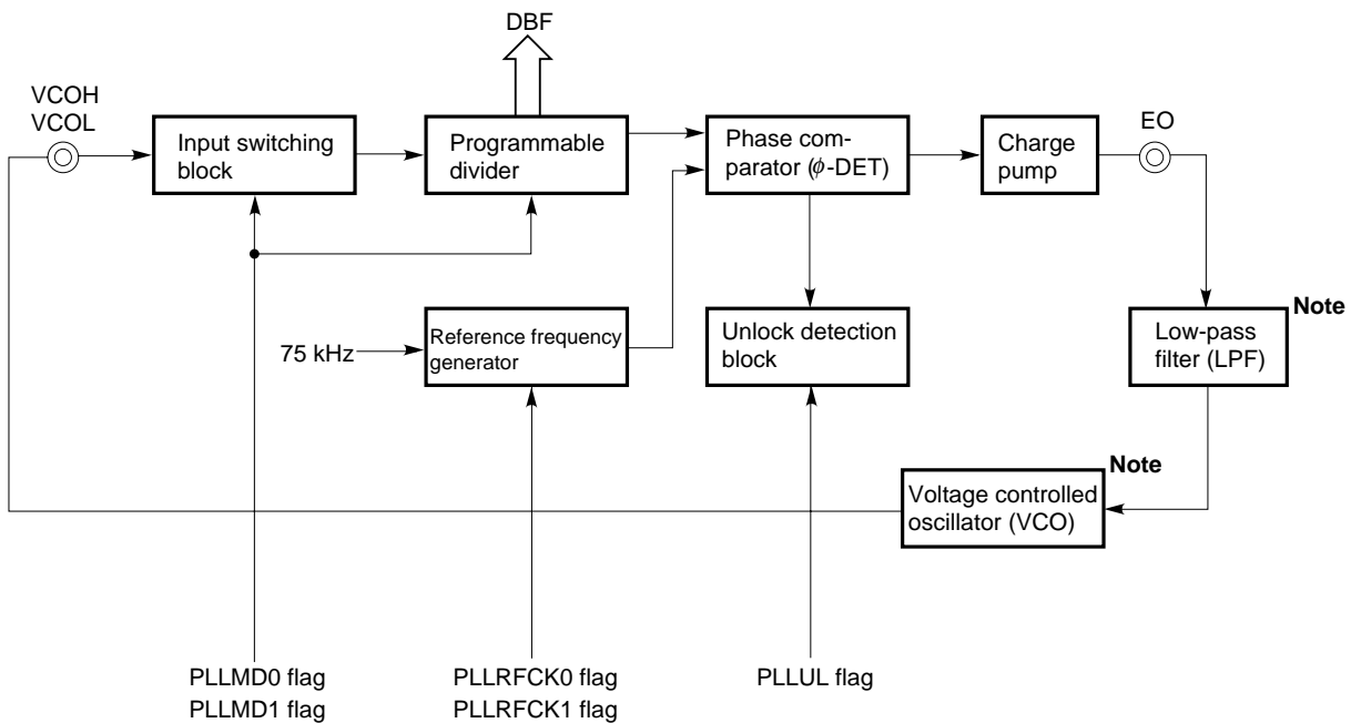
Fig. 11-1 PLL Frequency Synthesizer
