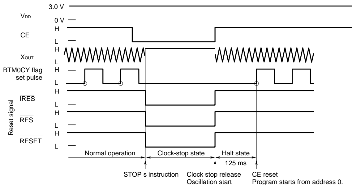
Fig. 15-5 CE Reset Operation When Clock-Stop Used
