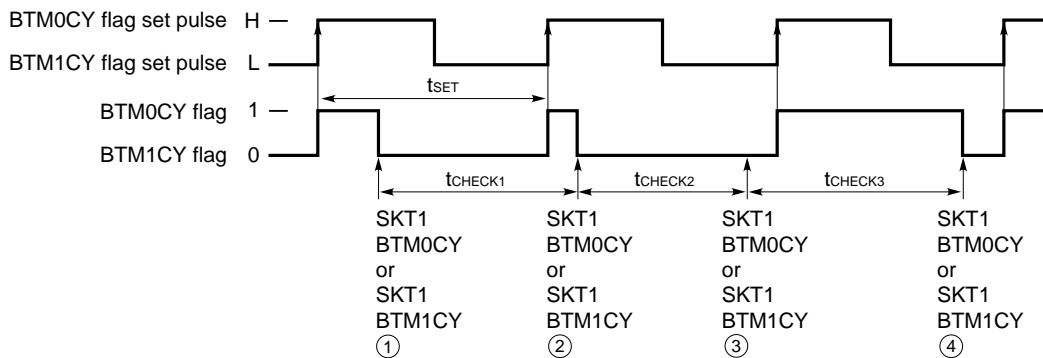
Fig. 10-4 Basic Timers 0 and 1 Error Related to the Detection Time of the BTM0CY and BTM1CY Flags
