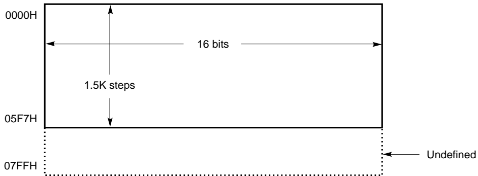
Fig. 2-2 Program Memory Configuration
