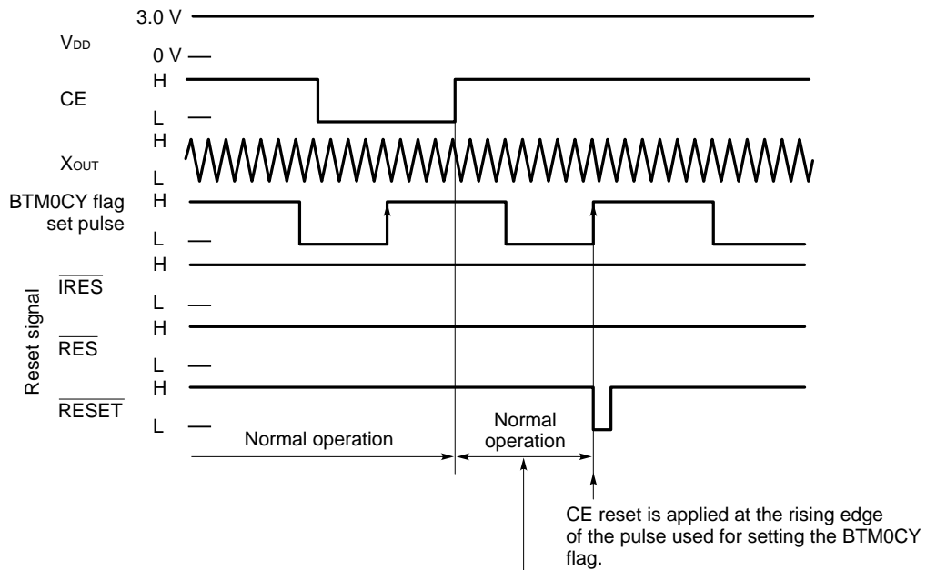
Fig. 15-4 CE Reset Operation When Clock-Stop Not Used
