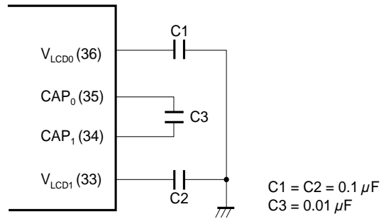
★ Fig. 13-2 Sample Doubler Configuration
