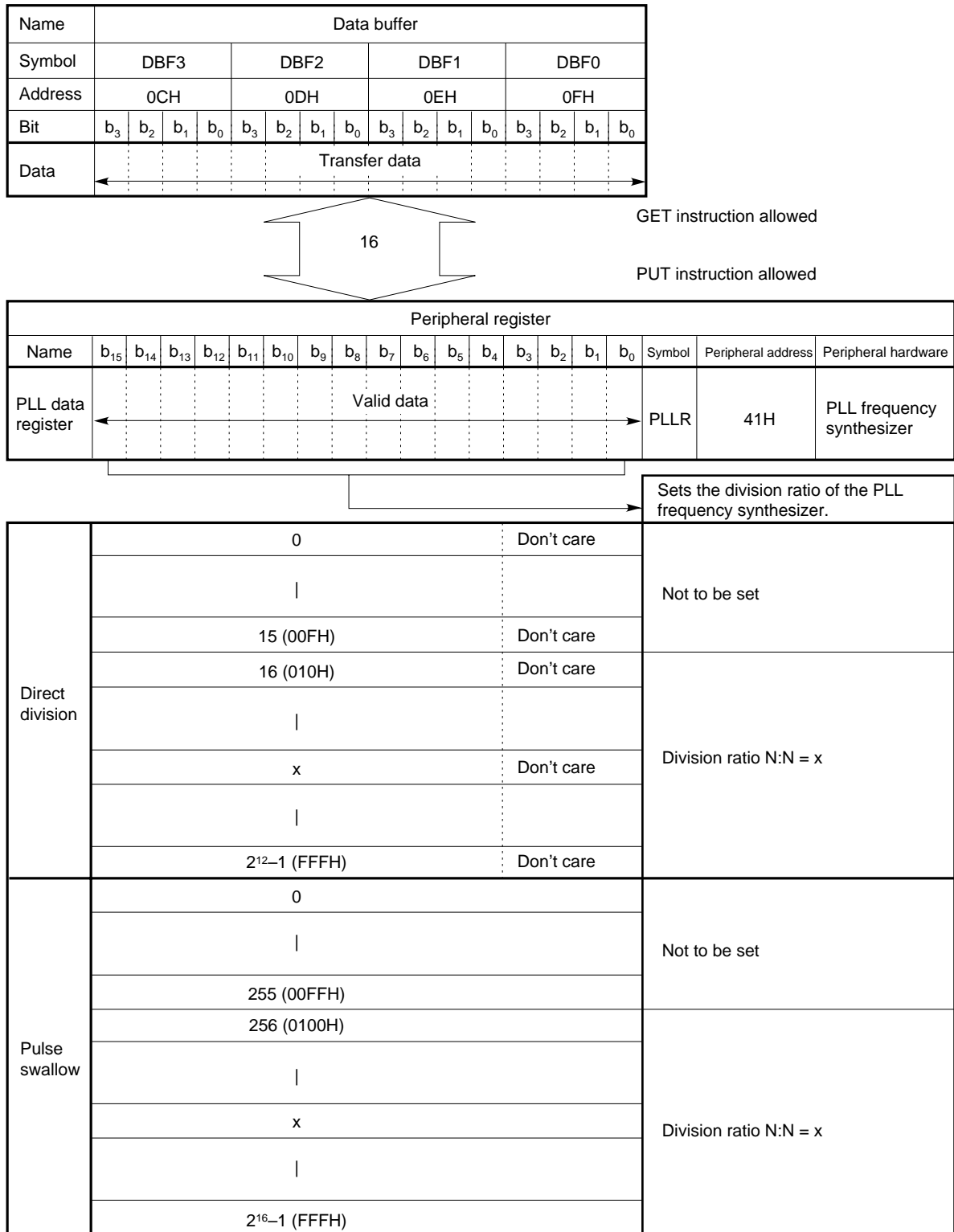
Fig. 11-4 Relationship between the PLL Data Register and Data Buffers
