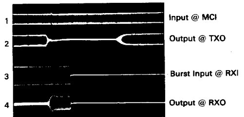
FIGURE 17 — IDLE-RECEIVE SWITCHING
