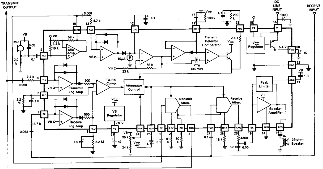
FIGURE 1 — TEST CIRCUIT
